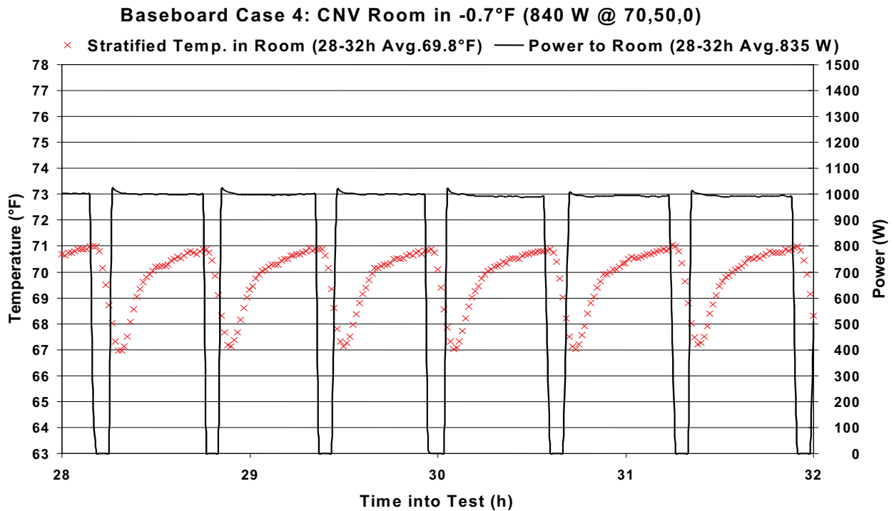
Figure 2. Example of Variation in Air Temperature and Heating Input Power for the Radiant Baseboard Heater in the Wood-Framed Room.
