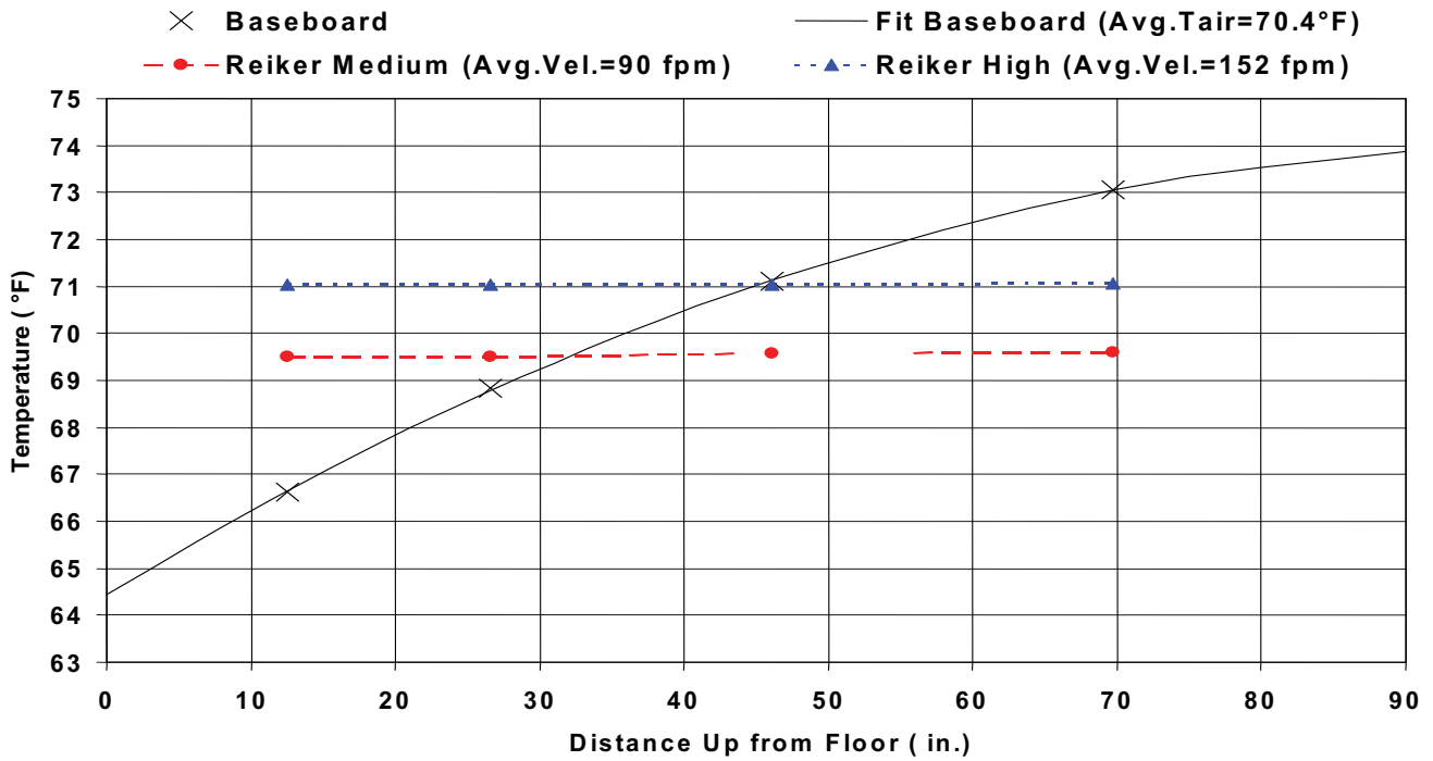
Figure 3. Stratification of Air Temperature from Floor to Ceiling of the Room from Structural Insulated Panels.
