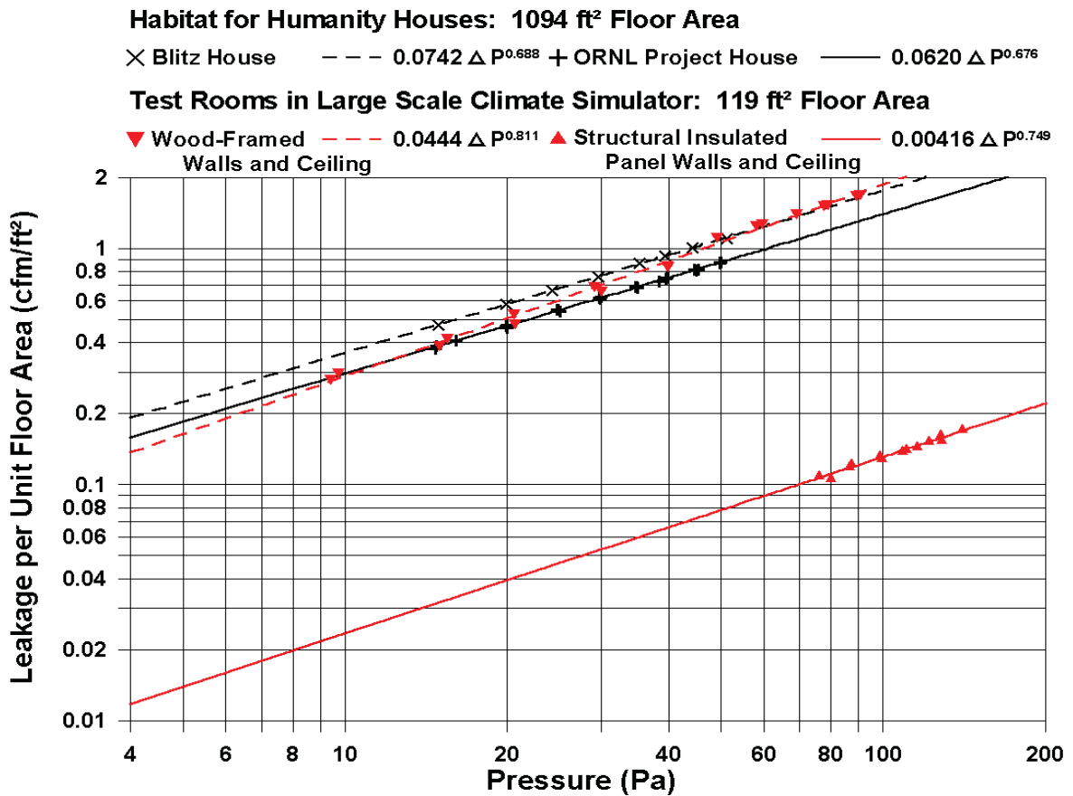
Figure 4. Blower Door Test Results for Whole Houses and the Test Rooms.
