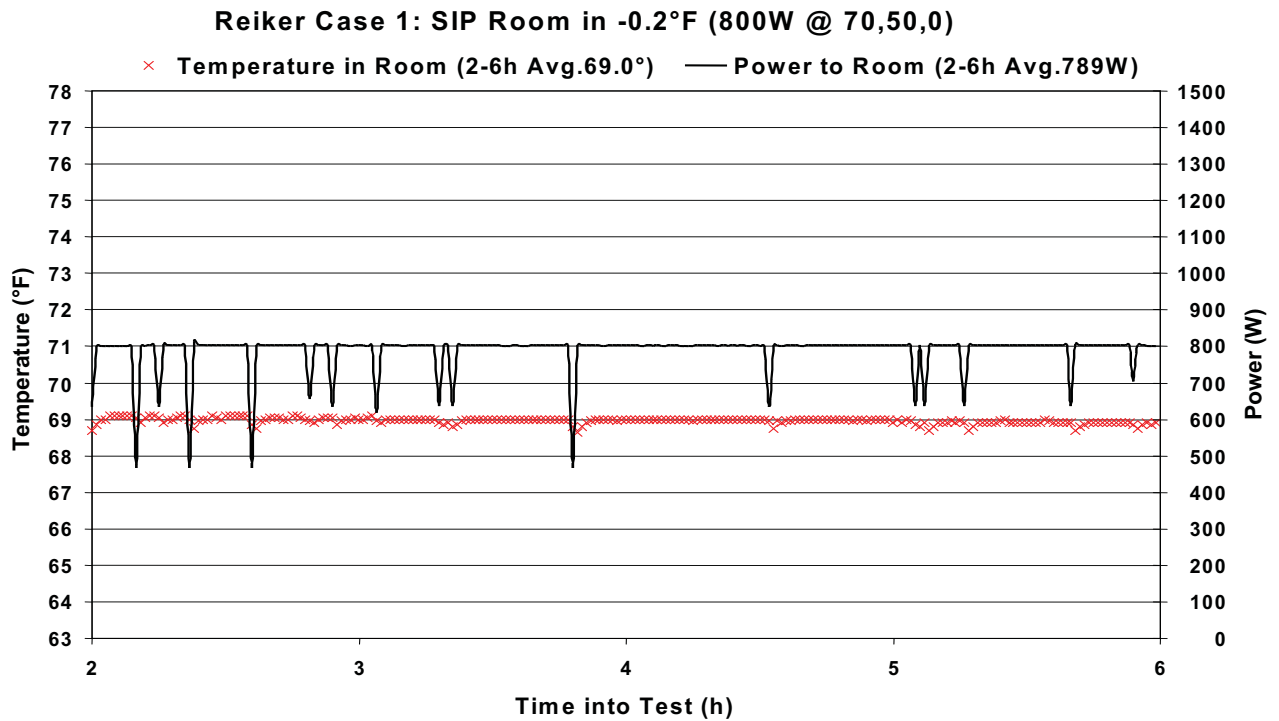
Figure 1. Example of Variation in Air Temperature and Heating Input Power for the Reiker Room Conditioner in the Room from Structural Insulated Panels.
